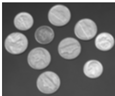
Filtered Image
