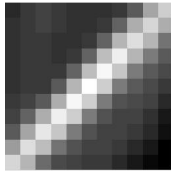
Restored PSF
