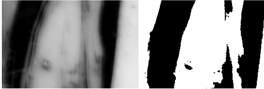
Original Image
