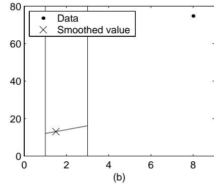
Loess Smoothing
